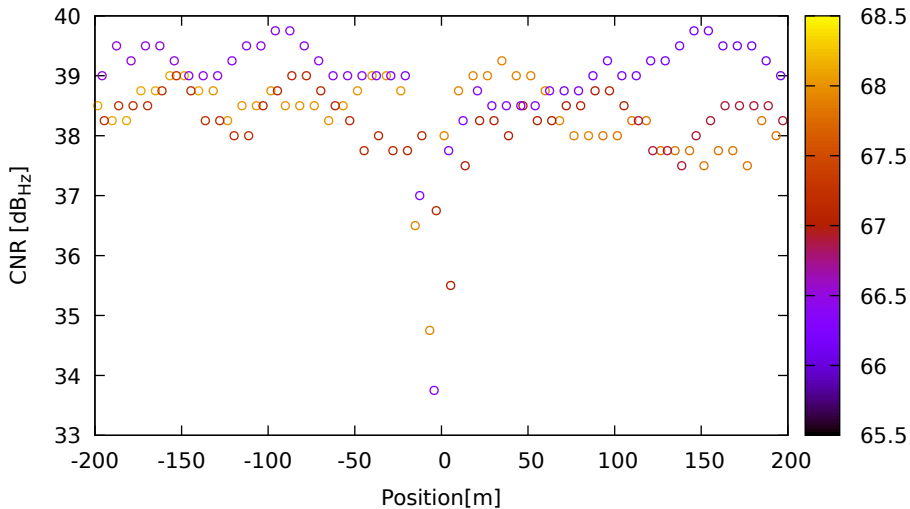
CNR vs position for R17 (G1) on XiaomiMi8 - DOY 263 jam. 3
