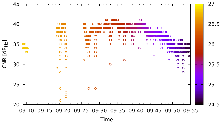
Timeline for C16 (B1) on HuaweiP40 - DOY 262
