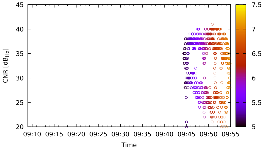
Timeline for C26 (B1) on HuaweiP40 - DOY 262
