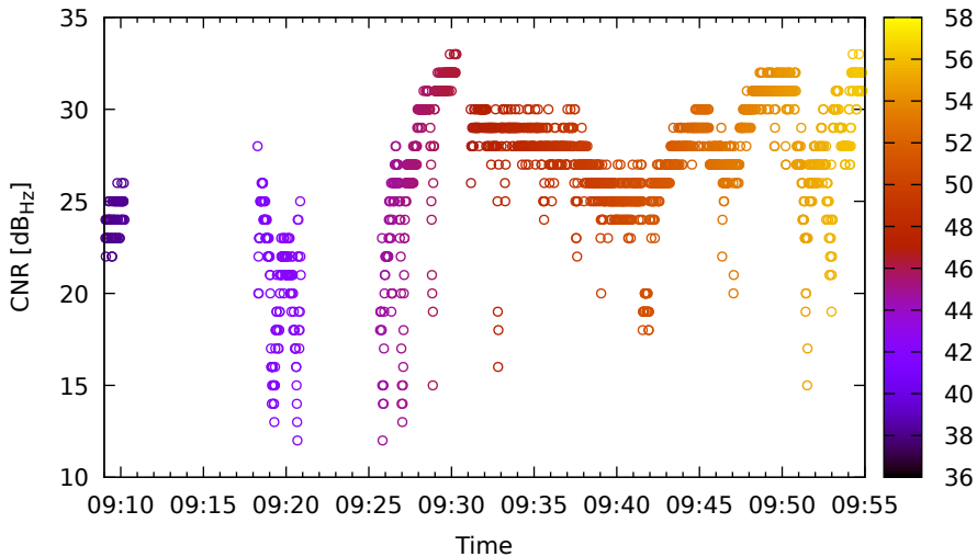
Timeline for E05 (E1) on HuaweiP40 - DOY 262
