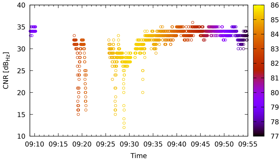
Timeline for G01 (L5) on HuaweiP40 - DOY 262
