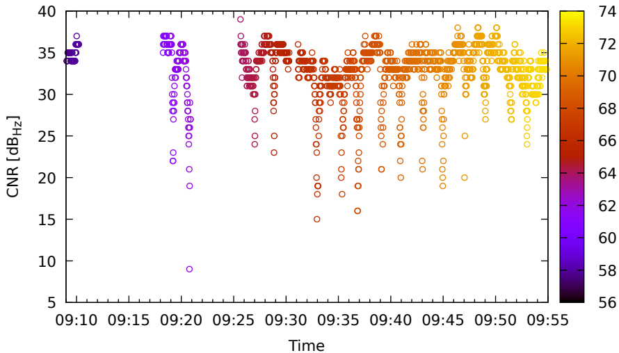
Timeline for G03 (L1) on HuaweiP40 - DOY 262
