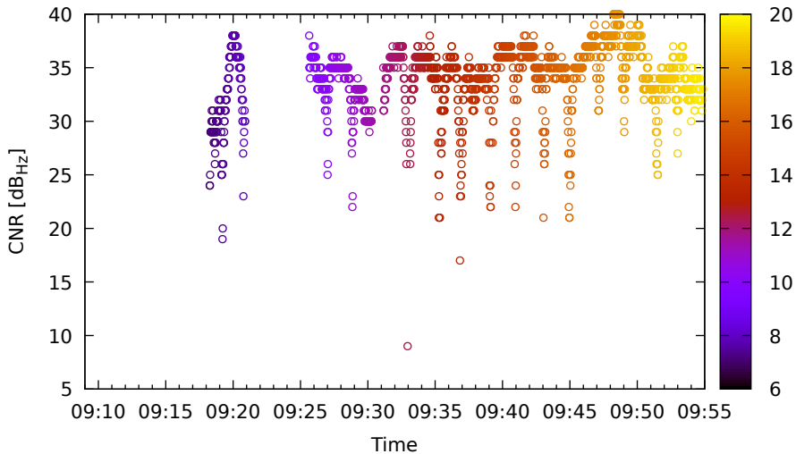
Timeline for G19 (L1) on HuaweiP40 - DOY 262
