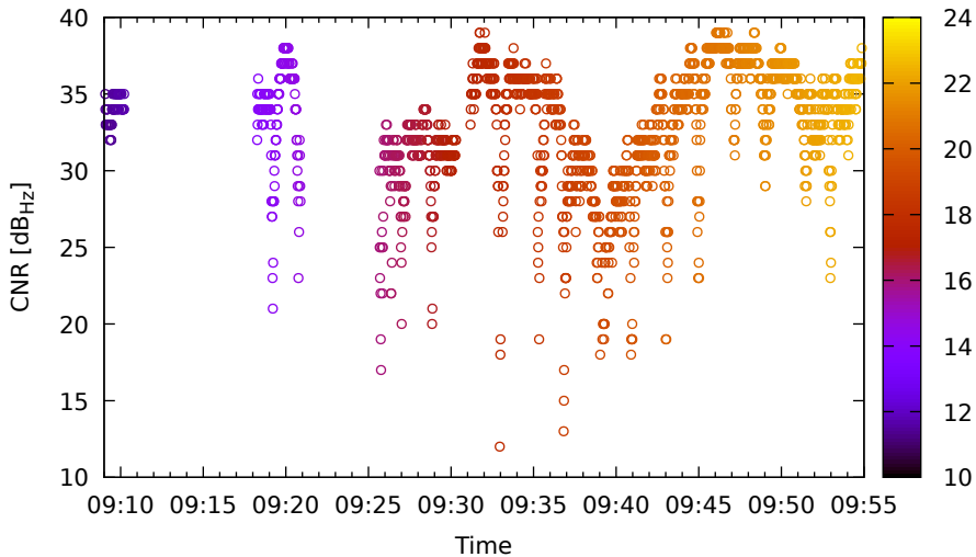
Timeline for G31 (L1) on HuaweiP40 - DOY 262
