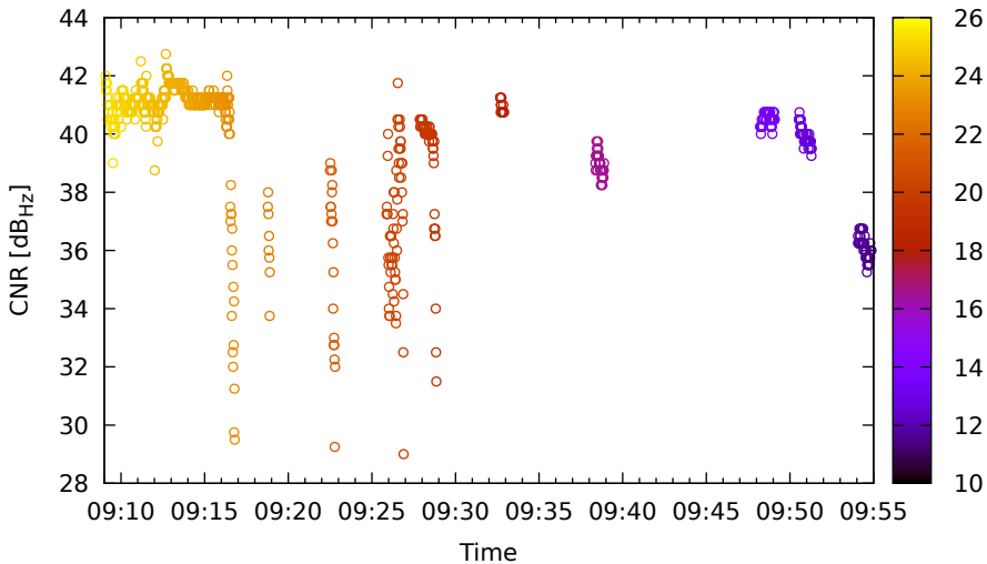
Timeline for E04 (E5) on LeicaGS15 - DOY 262
