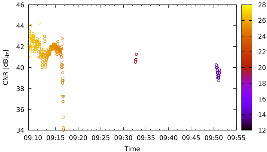
Timeline for E11 (E5a) on LeicaGS15 - DOY 262
