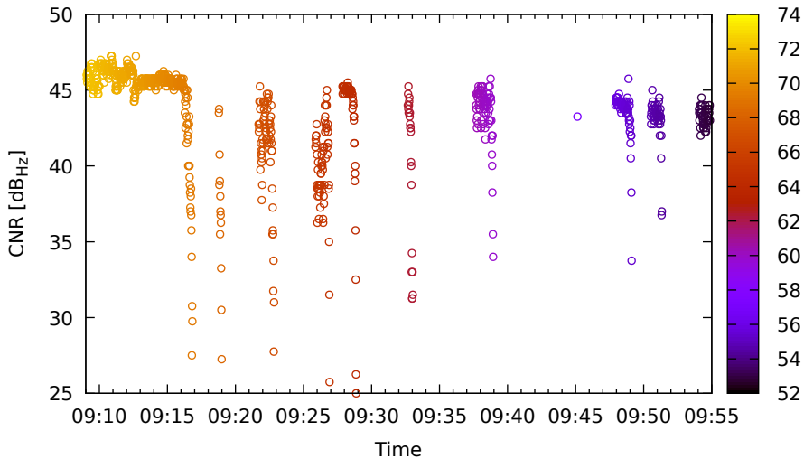
Timeline for G21 (L2) on LeicaGS15 - DOY 262
