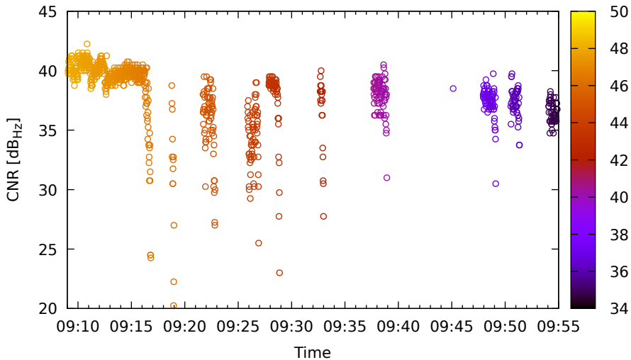
Timeline for G22 (L2) on LeicaGS15 - DOY 262
