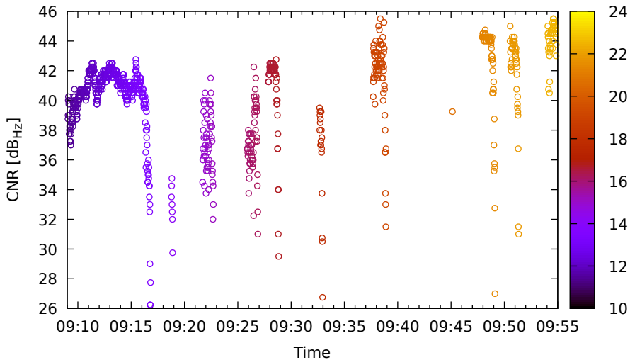
Timeline for G31 (L1) on LeicaGS15 - DOY 262
