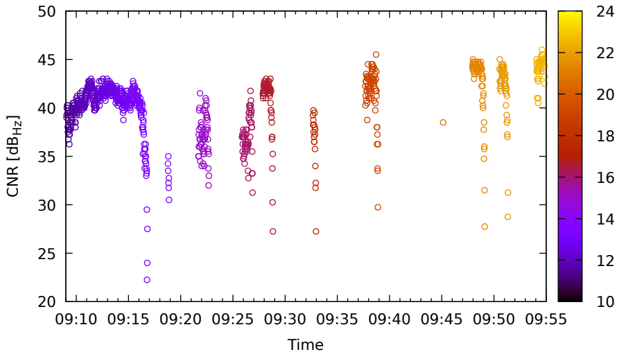
Timeline for G31 (L2) on LeicaGS15 - DOY 262
