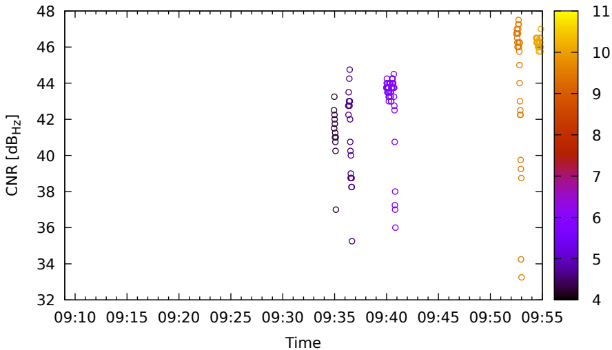
Timeline for E15 (E1) on LeicaGS15 - DOY 262
