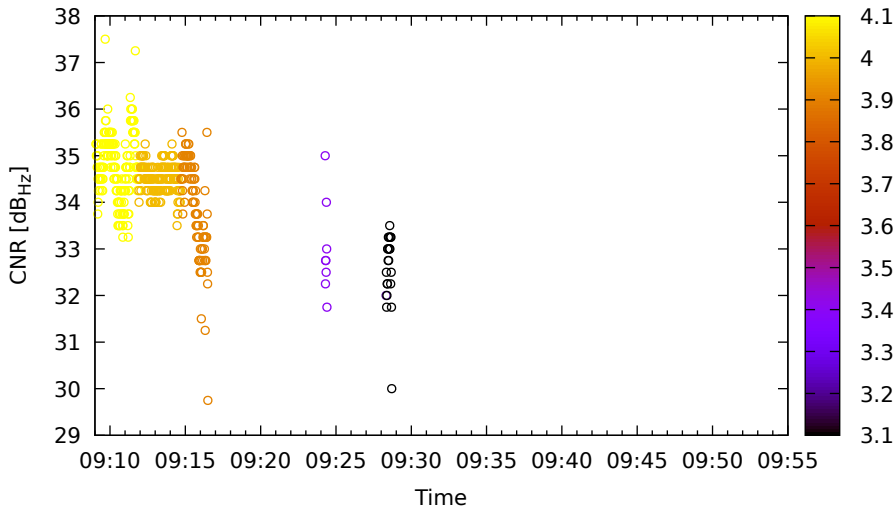
Timeline for E27 (E5) on LeicaGS15 - DOY 262
