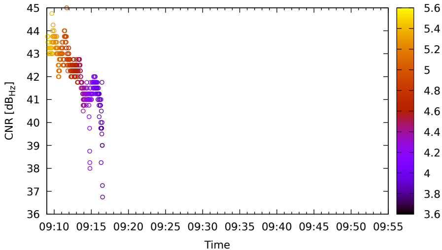
Timeline for E30 (E5b) on LeicaGS15 - DOY 262
