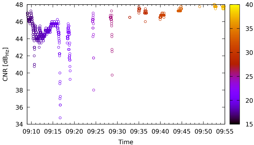
Timeline for G04 (L5) on LeicaGS15 - DOY 262
