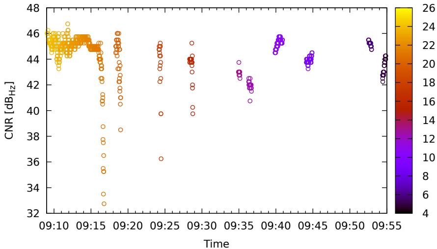
Timeline for G08 (L5) on LeicaGS15 - DOY 262
