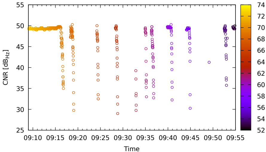
Timeline for G21 (L1) on LeicaGS15 - DOY 262
