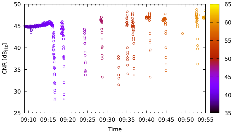
Timeline for R01 (G1) on LeicaGS15 - DOY 262
