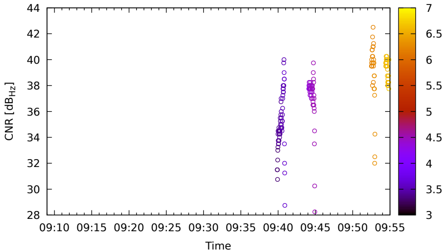
Timeline for R09 (G1) on LeicaGS15 - DOY 262
