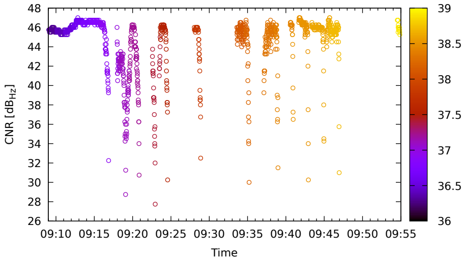
Timeline for C09 (B1) on LeicaGS18 - DOY 262
