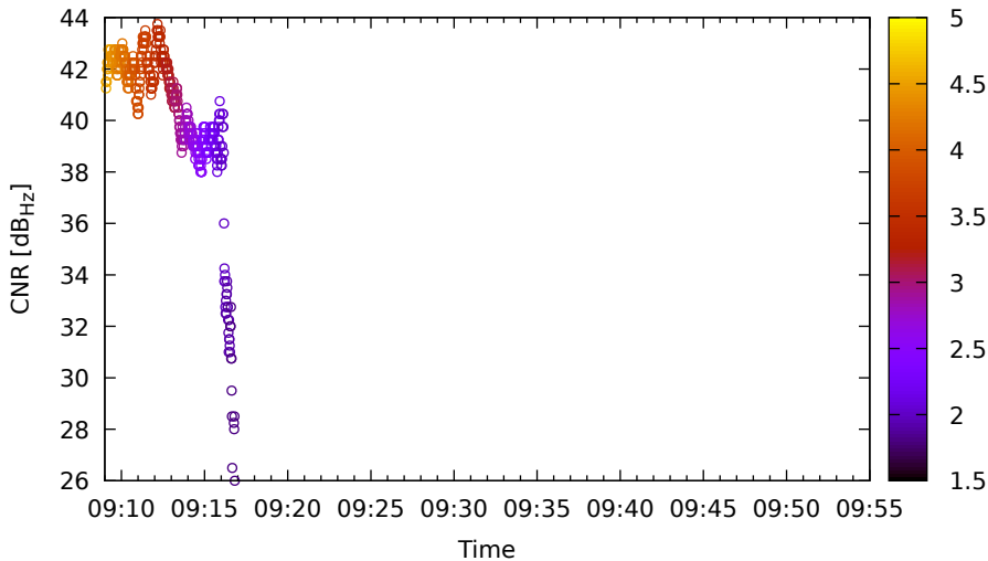
Timeline for C34 (B1) on LeicaGS18 - DOY 262
