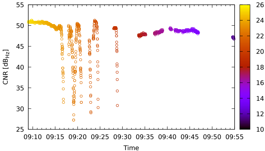
Timeline for E04 (E5) on LeicaGS18 - DOY 262
