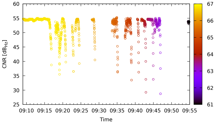
Timeline for E09 (E1) on LeicaGS18 - DOY 262
