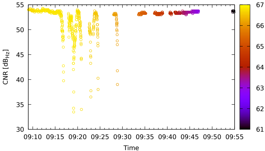
Timeline for E09 (E5a) on LeicaGS18 - DOY 262
