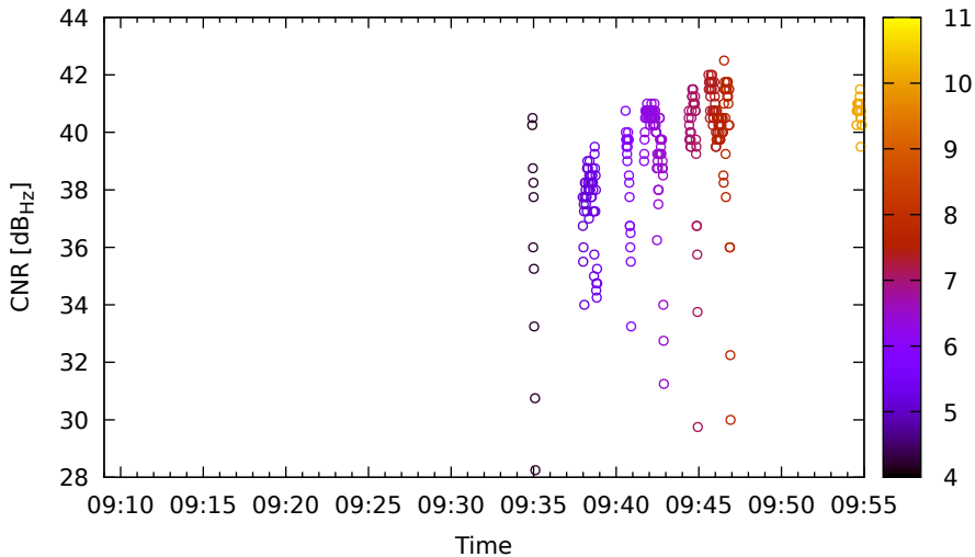
Timeline for E15 (E1) on LeicaGS18 - DOY 262
