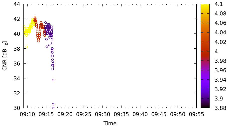
Timeline for E27 (E5b) on LeicaGS18 - DOY 262
