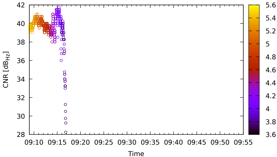
Timeline for E30 (E1) on LeicaGS18 - DOY 262
