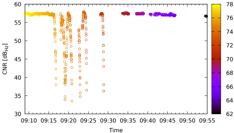
Timeline for E36 (E5) on LeicaGS18 - DOY 262
