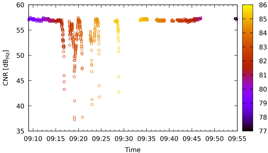
Timeline for G01 (L5) on LeicaGS18 - DOY 262
