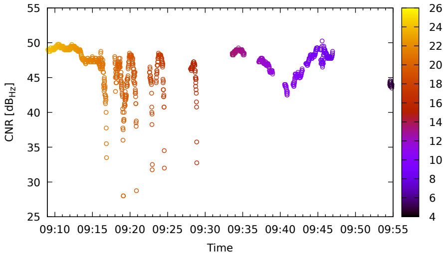
Timeline for G08 (L5) on LeicaGS18 - DOY 262
