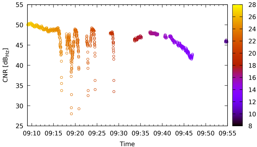
Timeline for G32 (L5) on LeicaGS18 - DOY 262
