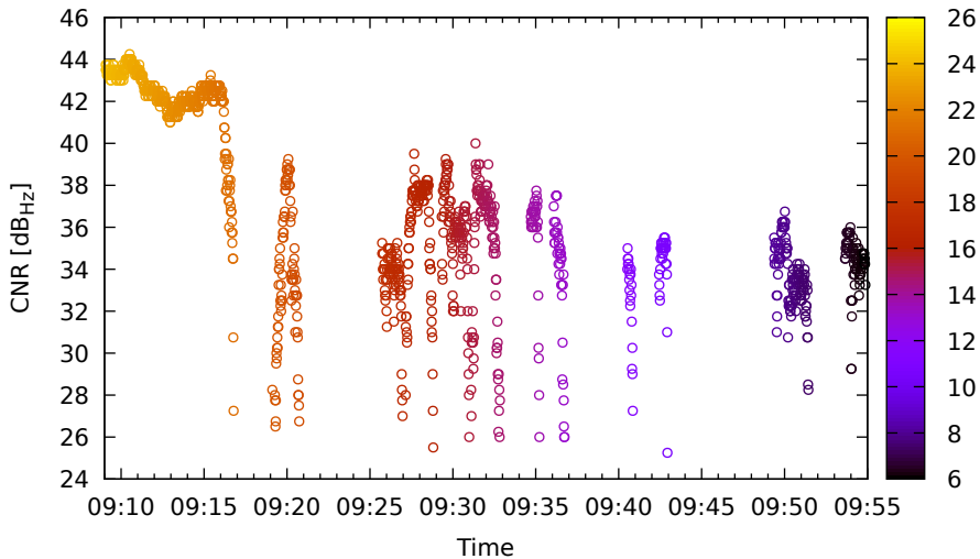
Timeline for C11 (B1) on LeicaGS18 - DOY 262
