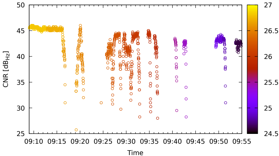
Timeline for C16 (B1) on LeicaGS18 - DOY 262
