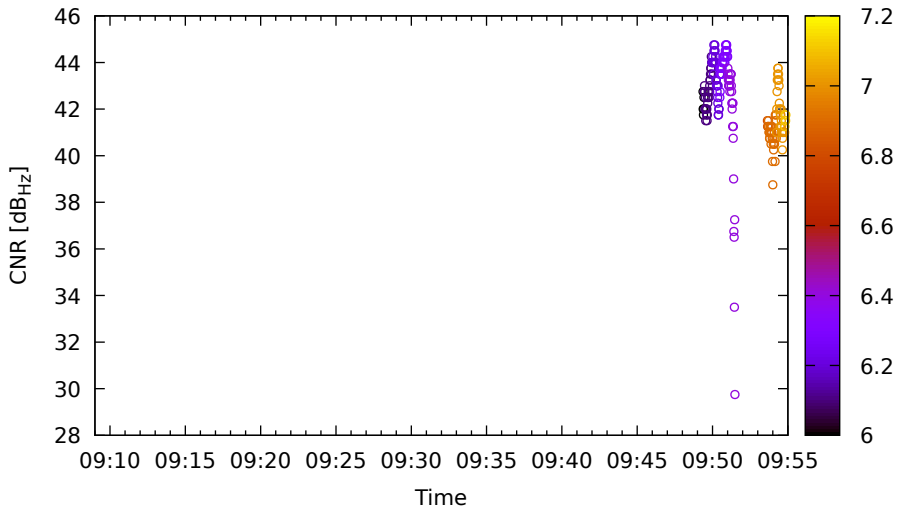
Timeline for C26 (B1) on LeicaGS18 - DOY 262
