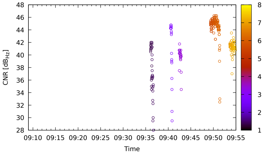
Timeline for E03 (E1) on LeicaGS18 - DOY 262
