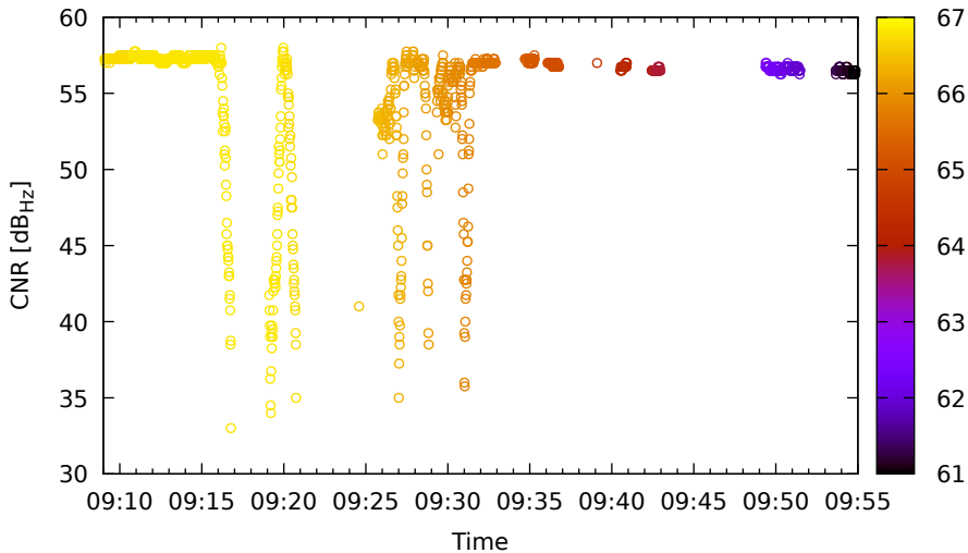
Timeline for E09 (E8) on LeicaGS18 - DOY 262
