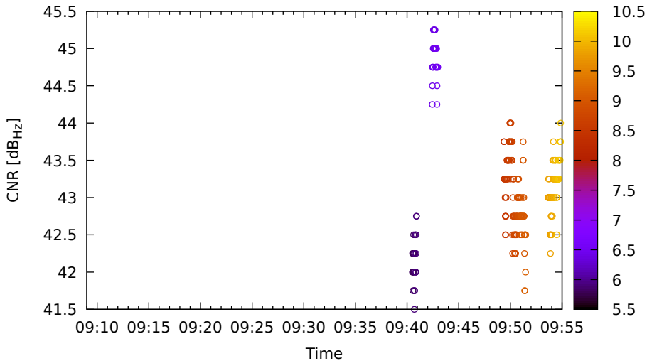
Timeline for E15 (E5a) on LeicaGS18 - DOY 262
