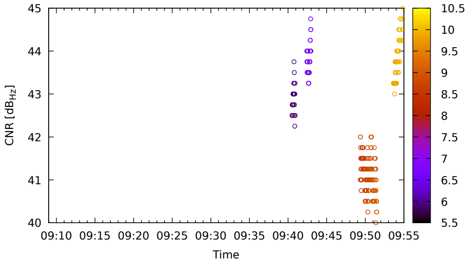
Timeline for E15 (E5b) on LeicaGS18 - DOY 262
