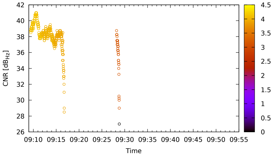
Timeline for E27 (E5b) on LeicaGS18 - DOY 262
