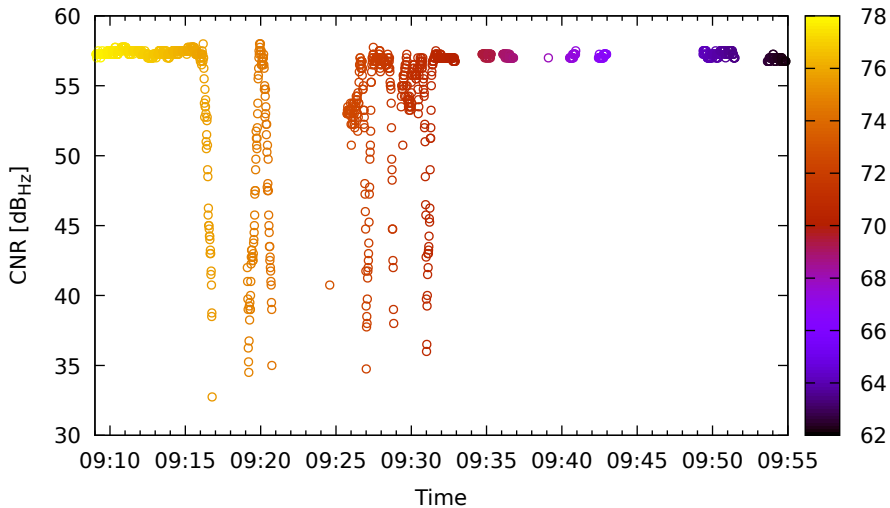
Timeline for E36 (E8) on LeicaGS18 - DOY 262
