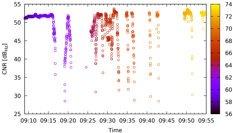
Timeline for G03 (L1) on LeicaGS18 - DOY 262
