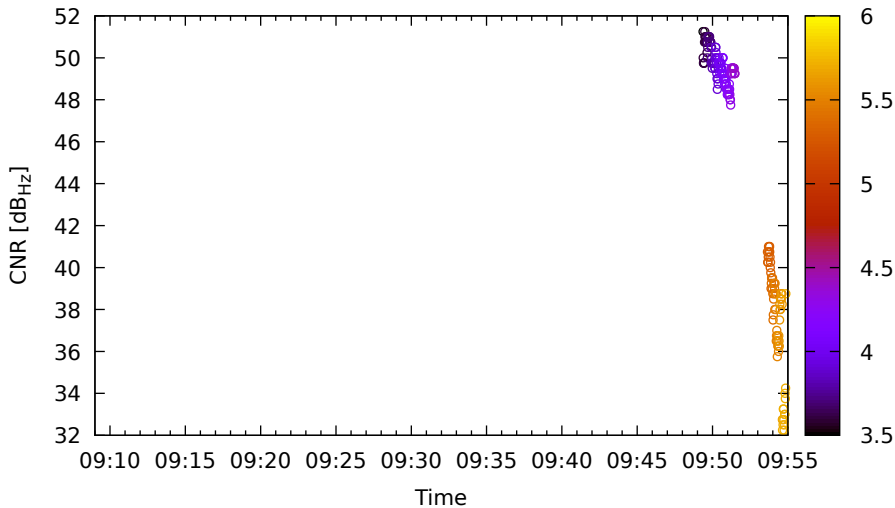
Timeline for G09 (L5) on LeicaGS18 - DOY 262
