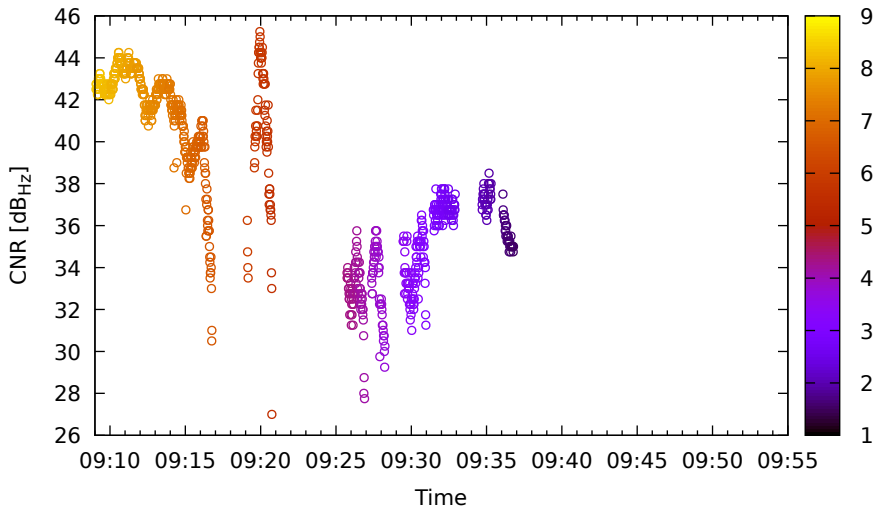
Timeline for G14 (L5) on LeicaGS18 - DOY 262
