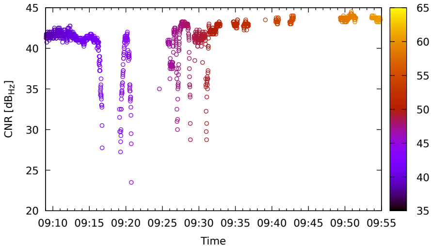
Timeline for R01 (G2) on LeicaGS18 - DOY 262
