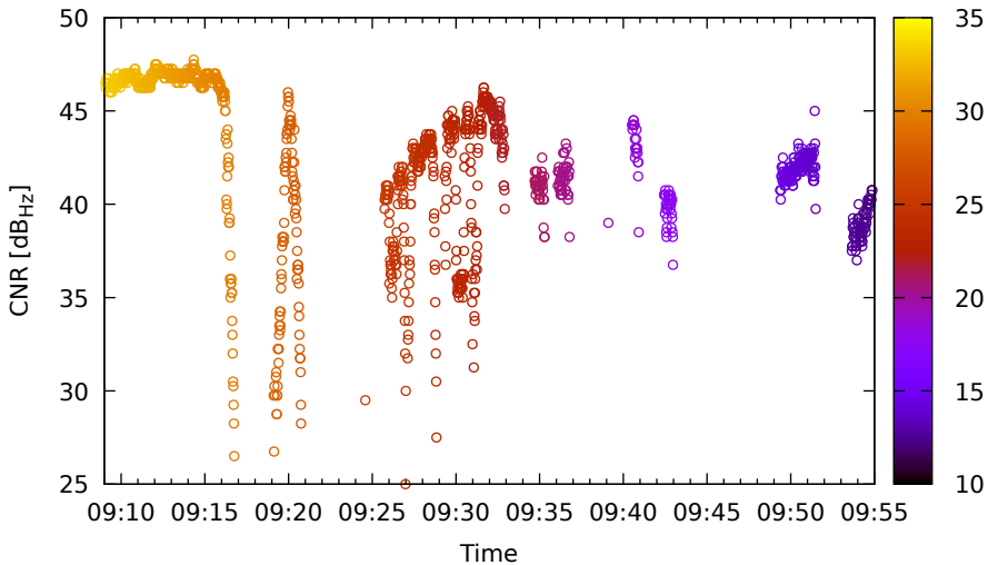
Timeline for R07 (G1) on LeicaGS18 - DOY 262
