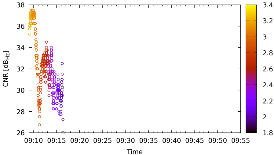
Timeline for R15 (G2) on LeicaGS18 - DOY 262
