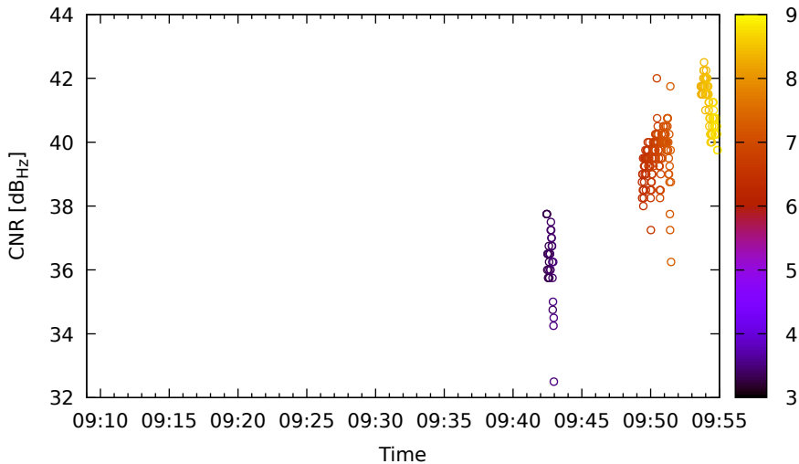
Timeline for R17 (G1) on LeicaGS18 - DOY 262
